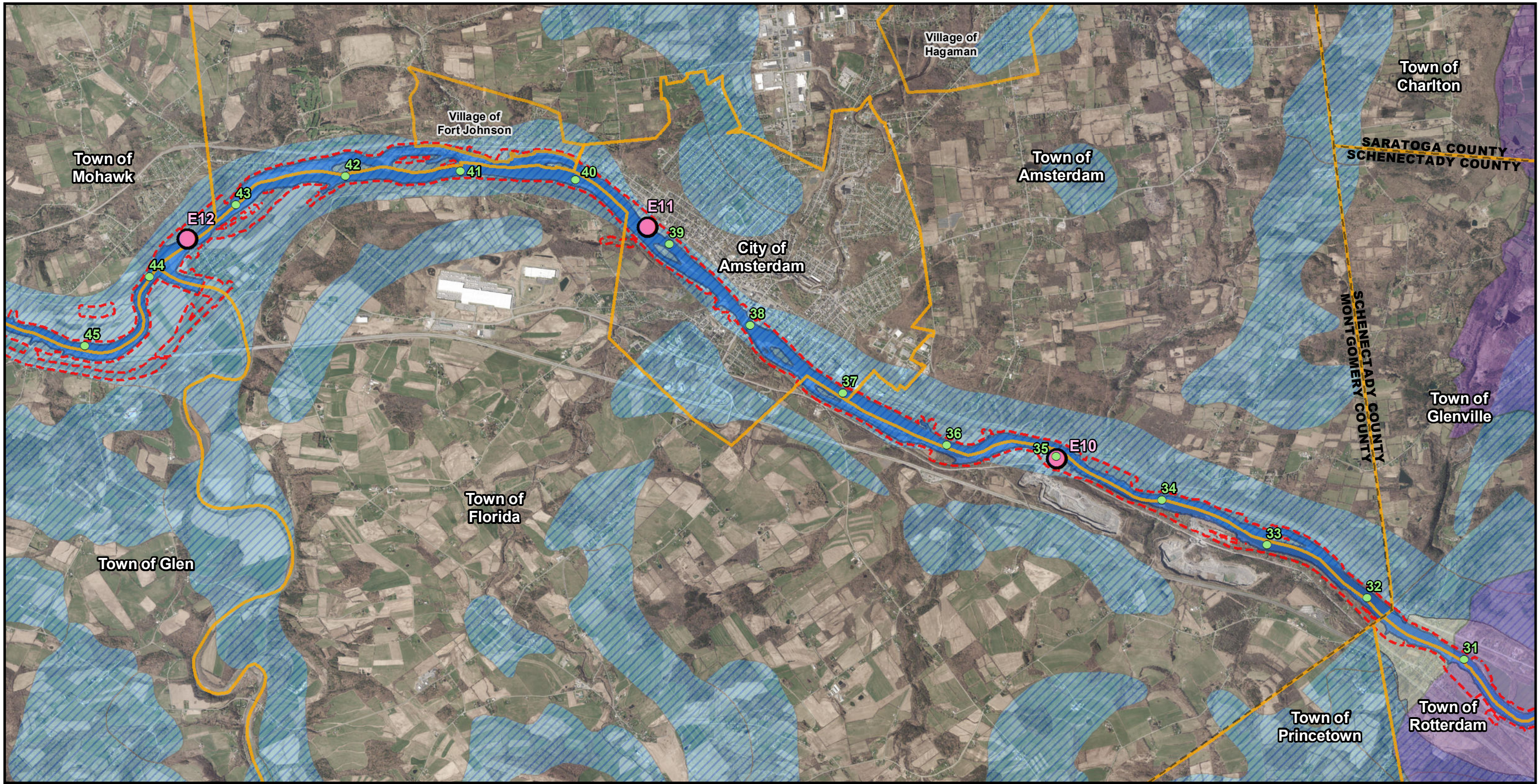
Figure 28F: Aquifers
